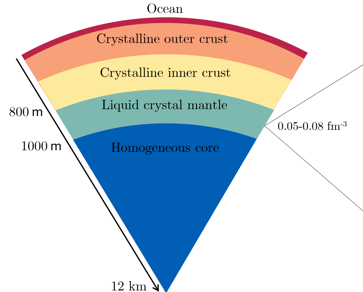
Neutron star schematic structure
