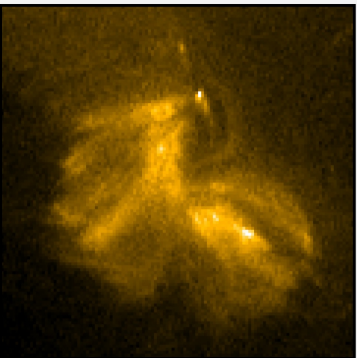
CBP from Solar Orbiter
