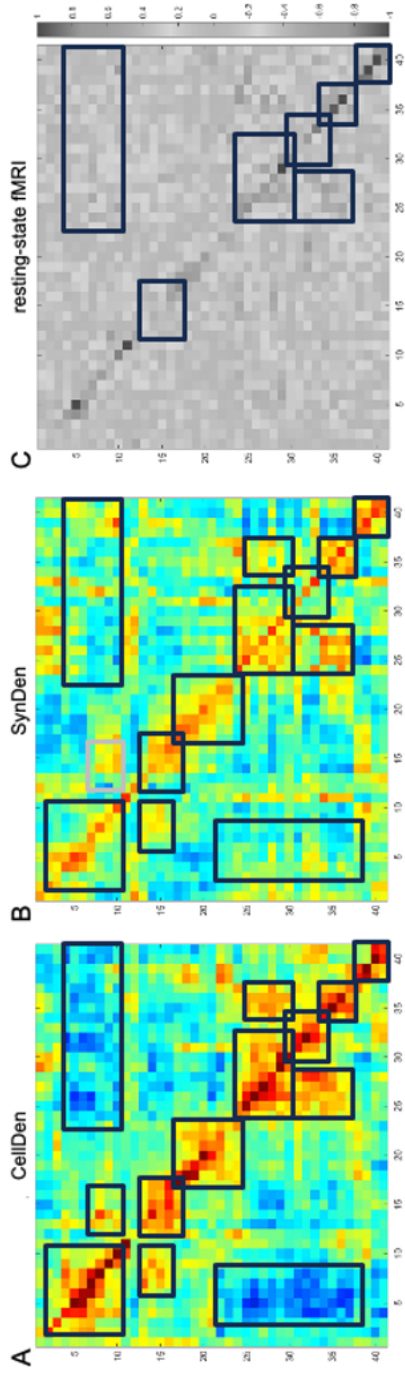
Figure 1. Correlated and anti-correlated networks by (A) CellDen, (B) SynDen, (C) resting fMRI.
