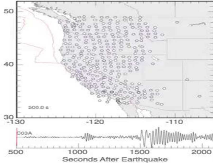
13 January, 2007 - East of Kuril Islands - Magnitude 8.1
